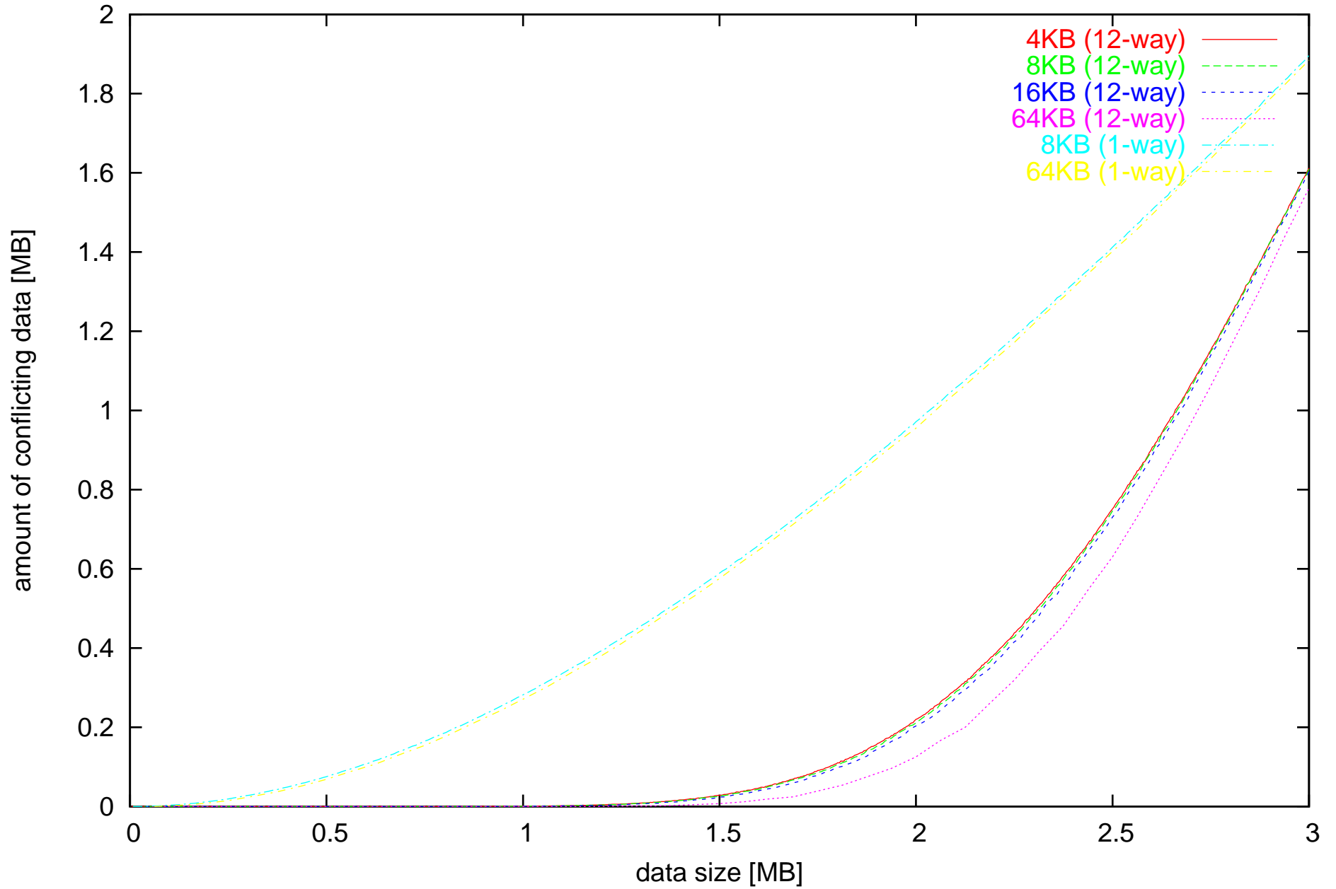
Avg. size of data exceeding cache associativity as a function of data size.
